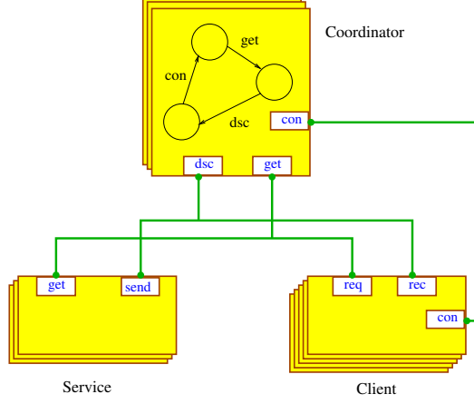
Figure 14: Request/Response architecture.
